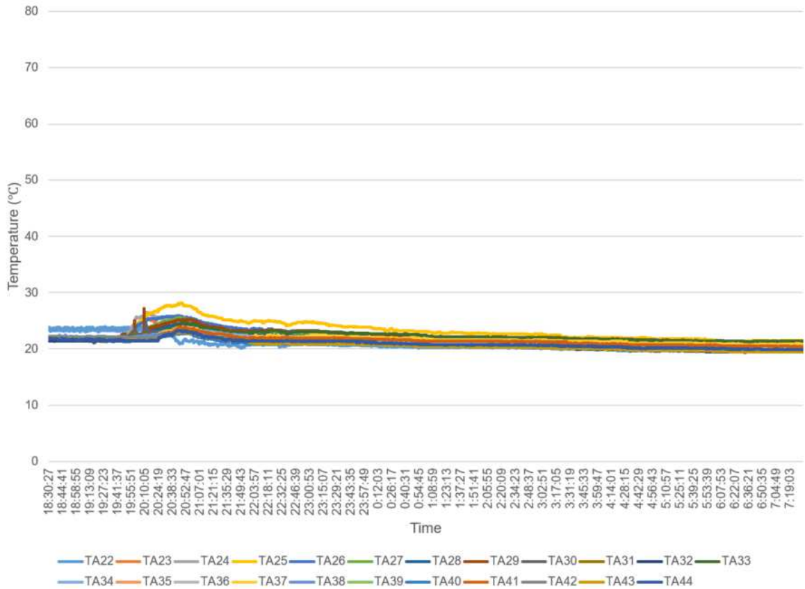
Figure 7. Temperature of instrumented wall B(Left side of initiating unit)
