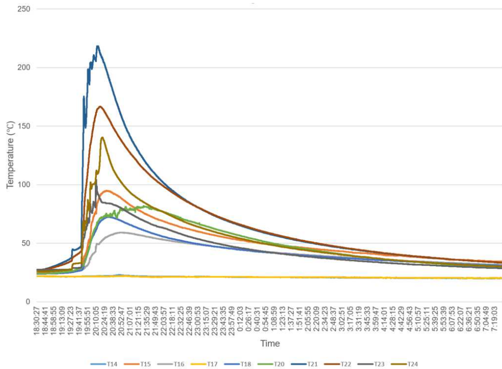
Figure 6. Temperature vs time curve of the initiating unit.
