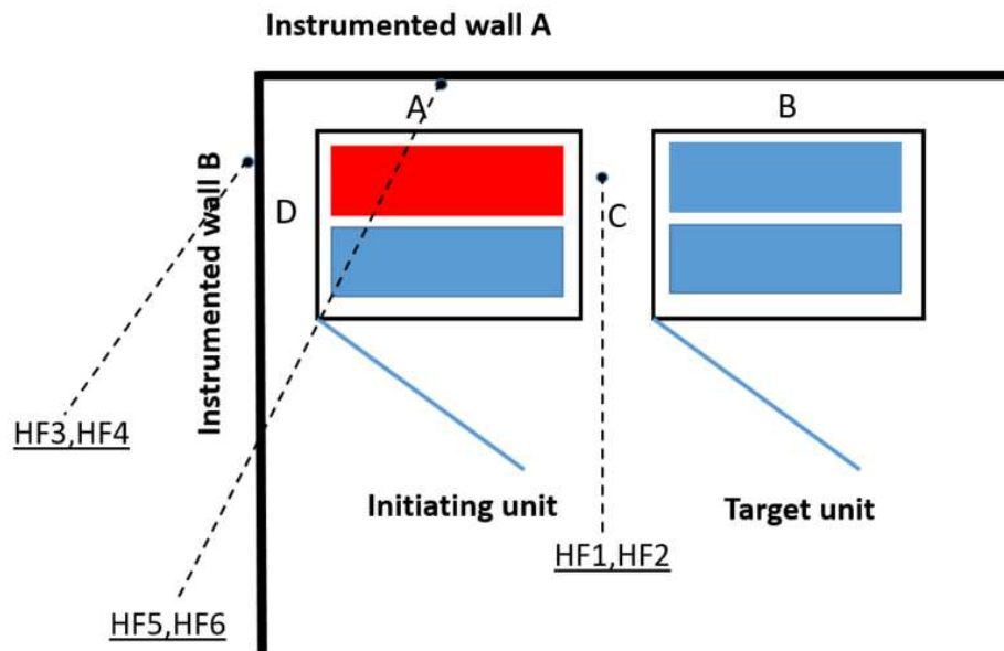
Figure 9. Heat flux sensor layout
