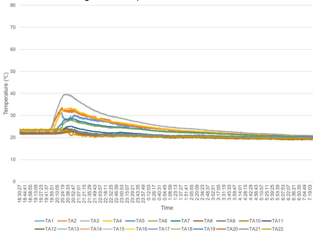
Figure 8. Temperature of instrumented wall A
