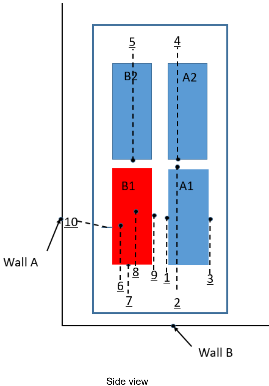
Figure 5. Surface temperatures of module in unit
