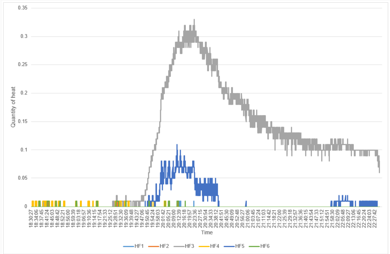
Figure 10. The measured heat flux of target walls and target unit
