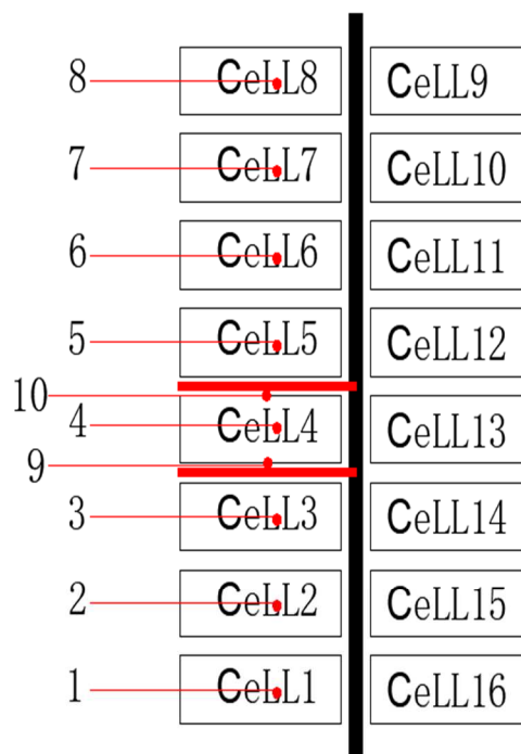
Figure 3: Thermocouple locations in module
