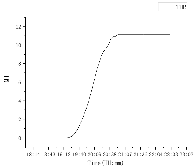
Figure 12 THR curve
