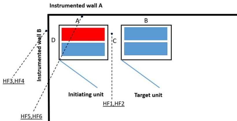
Figure 1. Top view of sub-unit's layout
