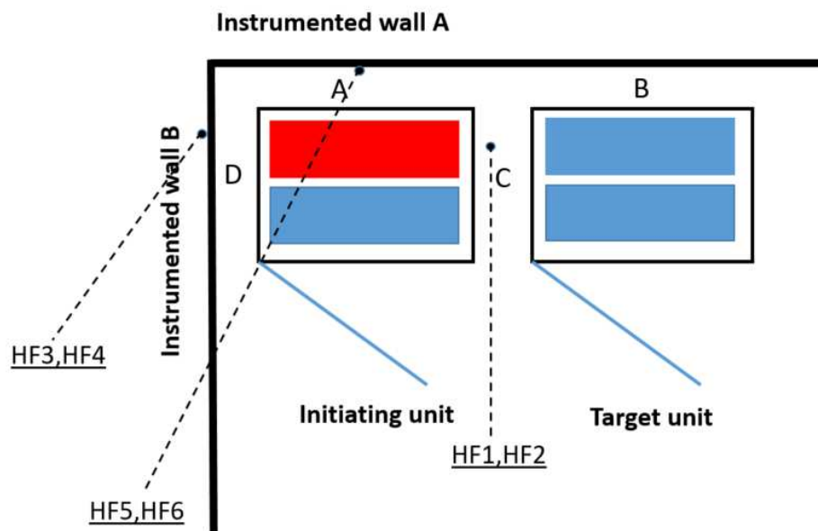
Figure 8. Heat flux sensor layout
