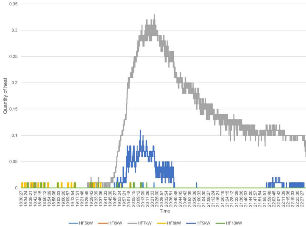
Figure 9. The measured heat flux of target walls and target unit
