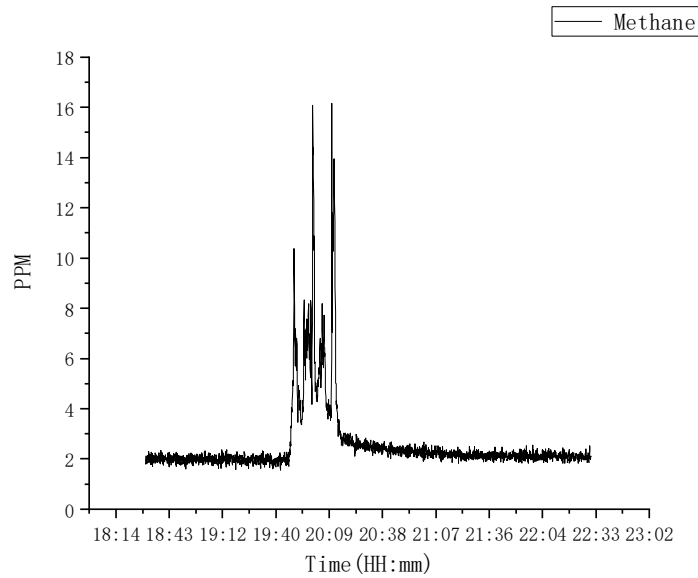
Figure 10 Hydrocarbon species:
